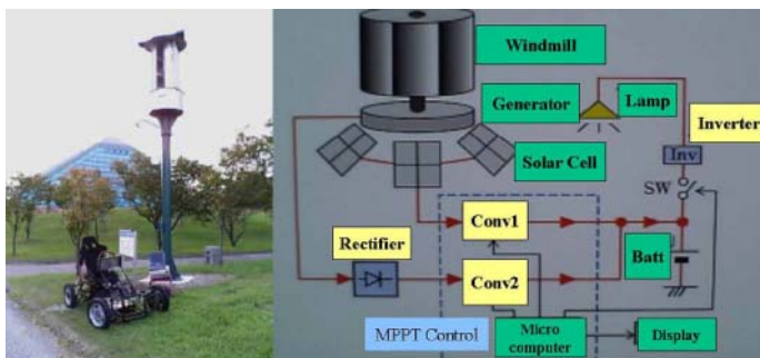
Figure 11 Self-powered street light (left), Power generating system (Right)
